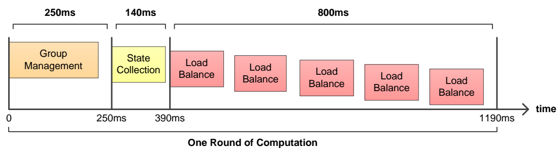
Figure 6.2: Round Robin Schedule
