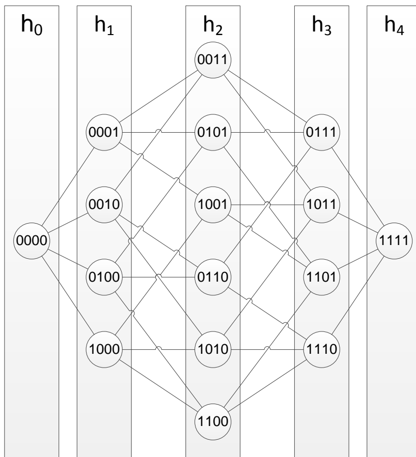
Figure 5.8: Example Hypercube
